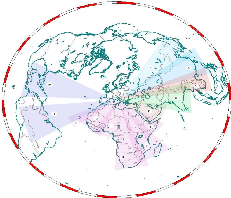
Target areas covered by directional antennas from SMG (for a larger view go to page 6)
